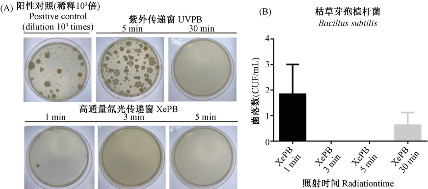
注:A:悬液涂布照射结果;阳性对照:阳性洗脱液稀释后铺板,培养 72 h;B:差异分析。 图 3 紫外传递窗和高通量氙光传递窗在不同照射时间点对枯草芽孢的杀灭情况 Note. A, Result of radiation. Positive control, The positive eluent was cultured 72 h after dilution. B, Difference analysis.
